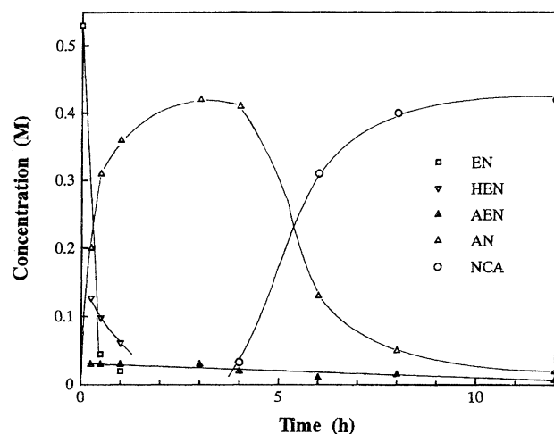
Fig. 1. Time profile of the products distribution in the Co-Mn-Br-catalyzed oxidation of 2-ethylnaphthalene in acetic acid at 90 °C. [Subst.]=0.53 M, (1 M=1 mol dm -3 ), [Subst.]:[Metal]:[NaBr]=100:4:8, [Co]:[Mn]=1:1 (molar ratio), atmospheric oxygen.
